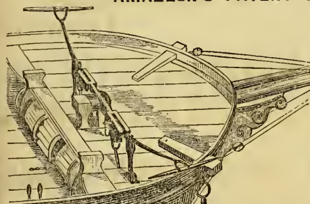
Amazeen's Patent Windlass Brake. Patented November 4, 1856.
